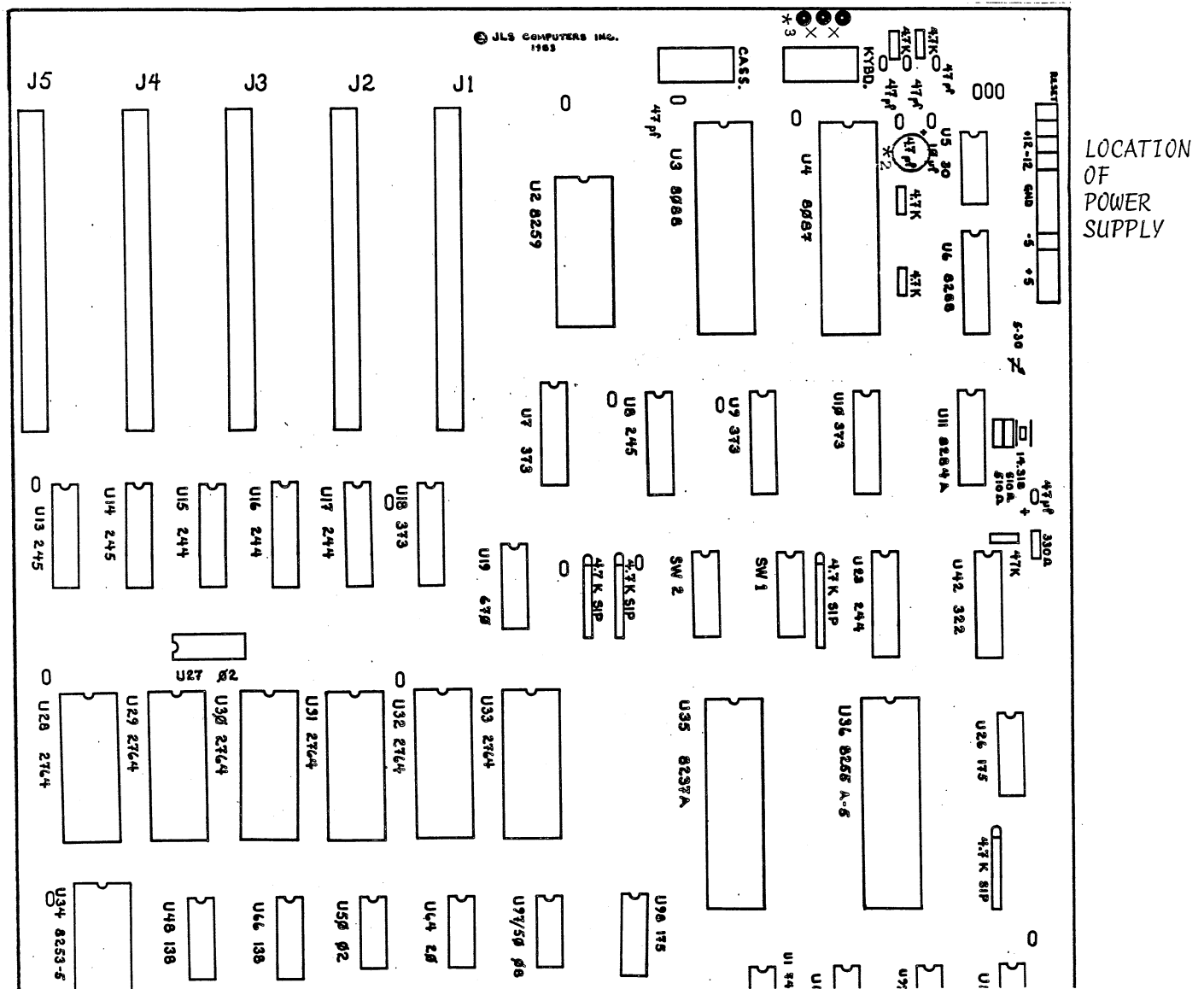
FIG. 5. A PORTION OF THE TOP VIEW OF THE MOTHERBOARD SHOWING FRONT-TO-BACK ORIENTATION AND LOCATION OF THE POWER SUPPLY.
