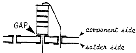
FIG. 4. INSTALLING A RESISTOR ON ITS END.
