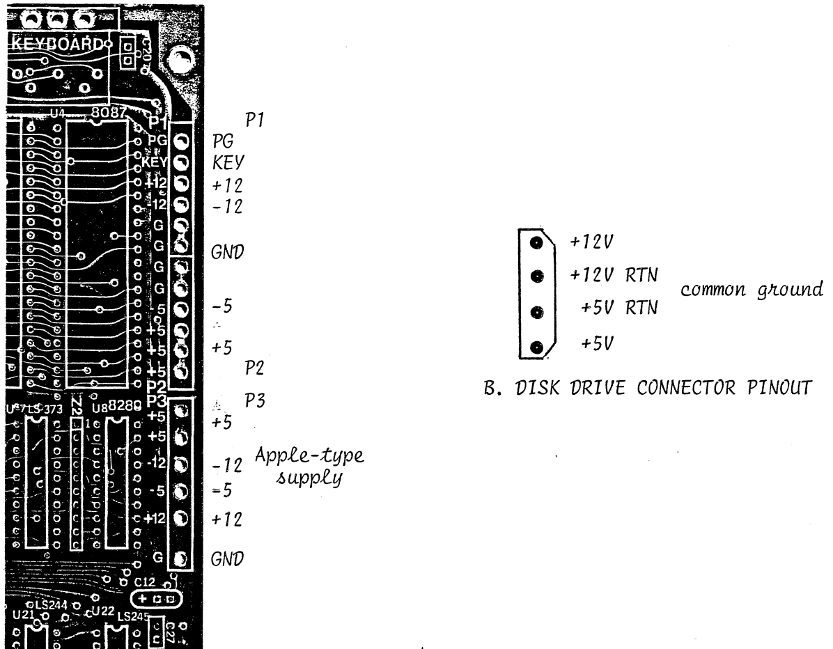
A. MOTHERBOARD POWER SUPPLY PINOUT
