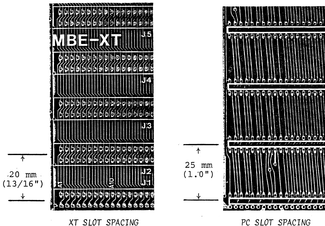
FIG. 8. XT AND PC MOTHERBOARD SLOT SPACING (center-to-center)
